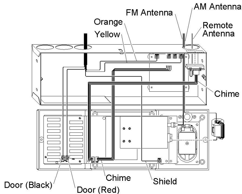
Figure 10 - dmc1 connections
