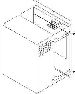
Figure 17 – Amplifier mounting
