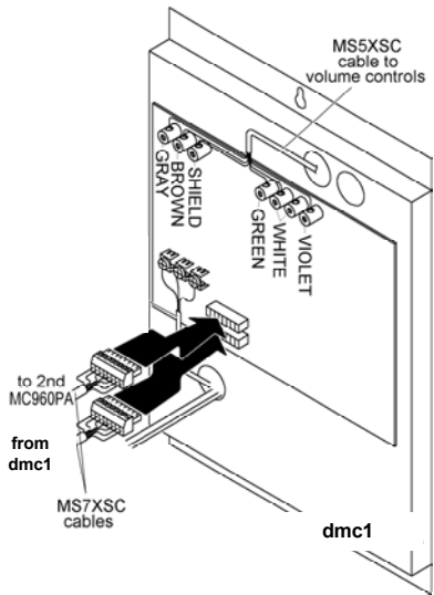
Figure 19 – Wiring connections
