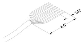
Figure 1 - CAT5 wire
