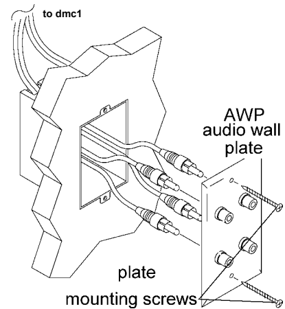
Figure 5 - External source wiring
