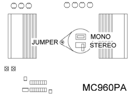
Figure 20 – Jumper connections
