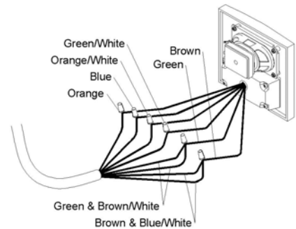
Figure 3 – Patio station wiring connections
