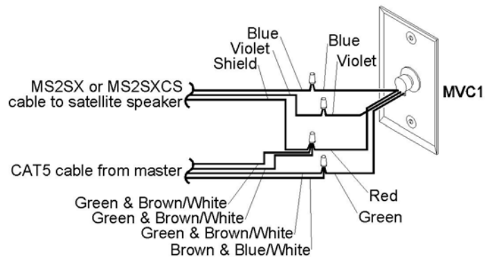
Figure 4 - Volume control wiring
